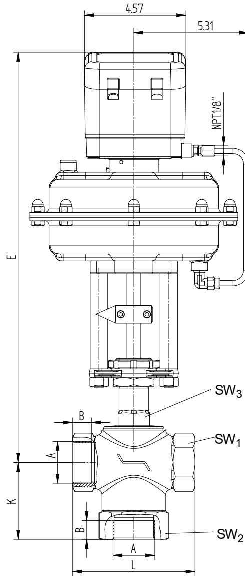
diaphragm actuator with digital positioner Type 8049
