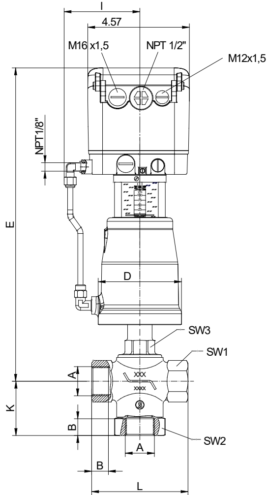
digital positioner Type 8049
